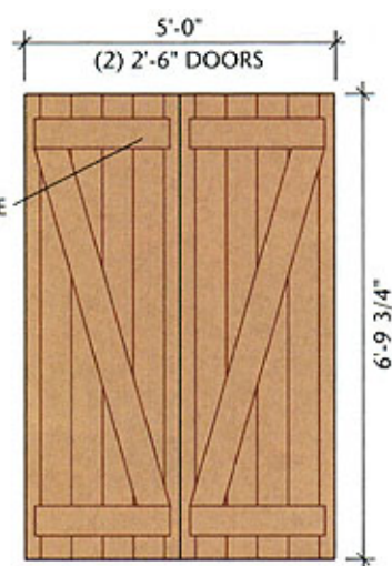
INSIDE ELEVATION
